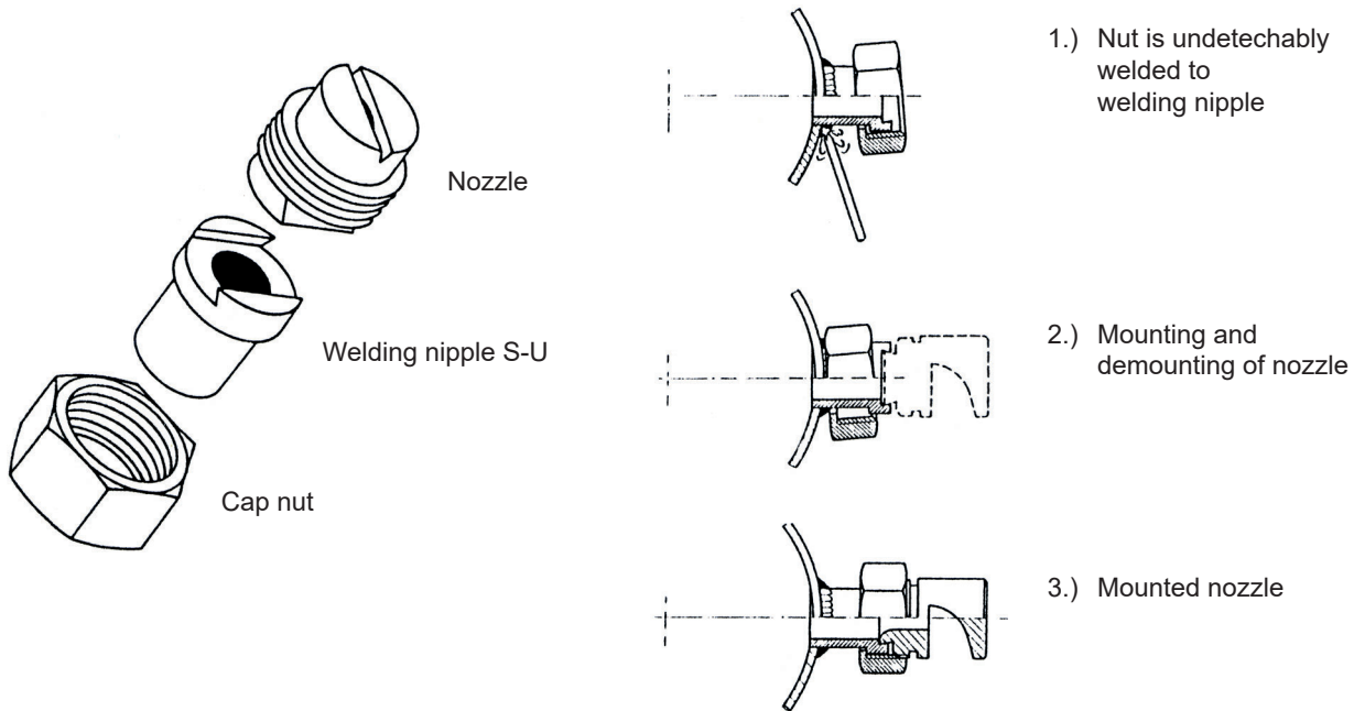
Welding nipple S-U
