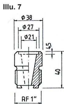
Variant A Adapter S3 - A
