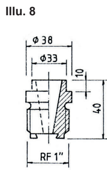
Variant B Adapter S3 - B
