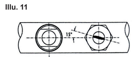
Flat fan nozzles offset by 15°
