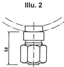
Variant B with welding nipple and pipe radius
