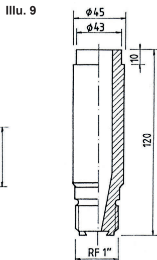
Variant C Adapter S3 - C
