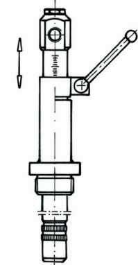
Nozzle lance with sliding sleeve and head thread, on request
