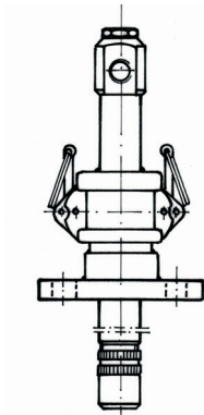
Nozzle lance with camloc fastener, fixed or with combined sliding sleeve
