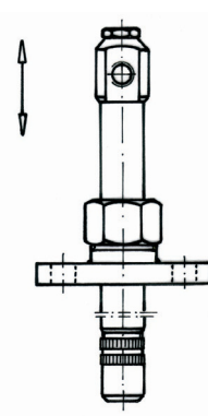
Nozzle lance with collet and sealing for pressure containers, slidable
