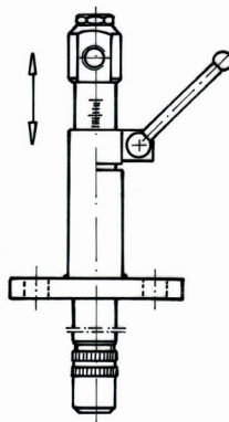
Nozzle lance with sliding sleeve and flange at choice, standard 120 mm Ø
