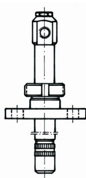
Nozzle lance with screw connection, fixed or slidable DIN 11851 and DIN 11864-1
