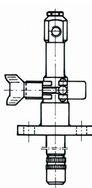
Nozzle lance with sold clamp and clamping nipples, fixed or with sliding sleeve
