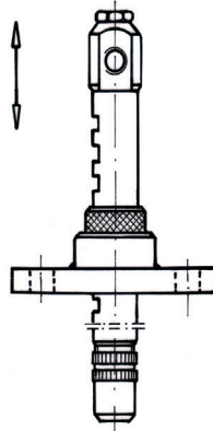
Nozzle lance with integrated height adjustment by means of a clampable adjusting disk, compatible with systems on the market
