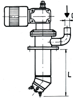
Type AT-GE 70 - 90° with elec. worm gear
