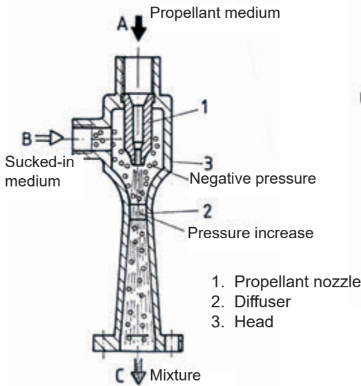
Type JP with flange connection (see tables)
