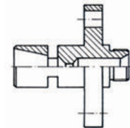
Type JM-F with flange connection to flange to in- or outside of container, Dimensions on request
