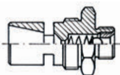
Type JM-KR with head thread and integrated check valve, Dimensions on request
