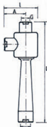
Type JVP with thread connection
